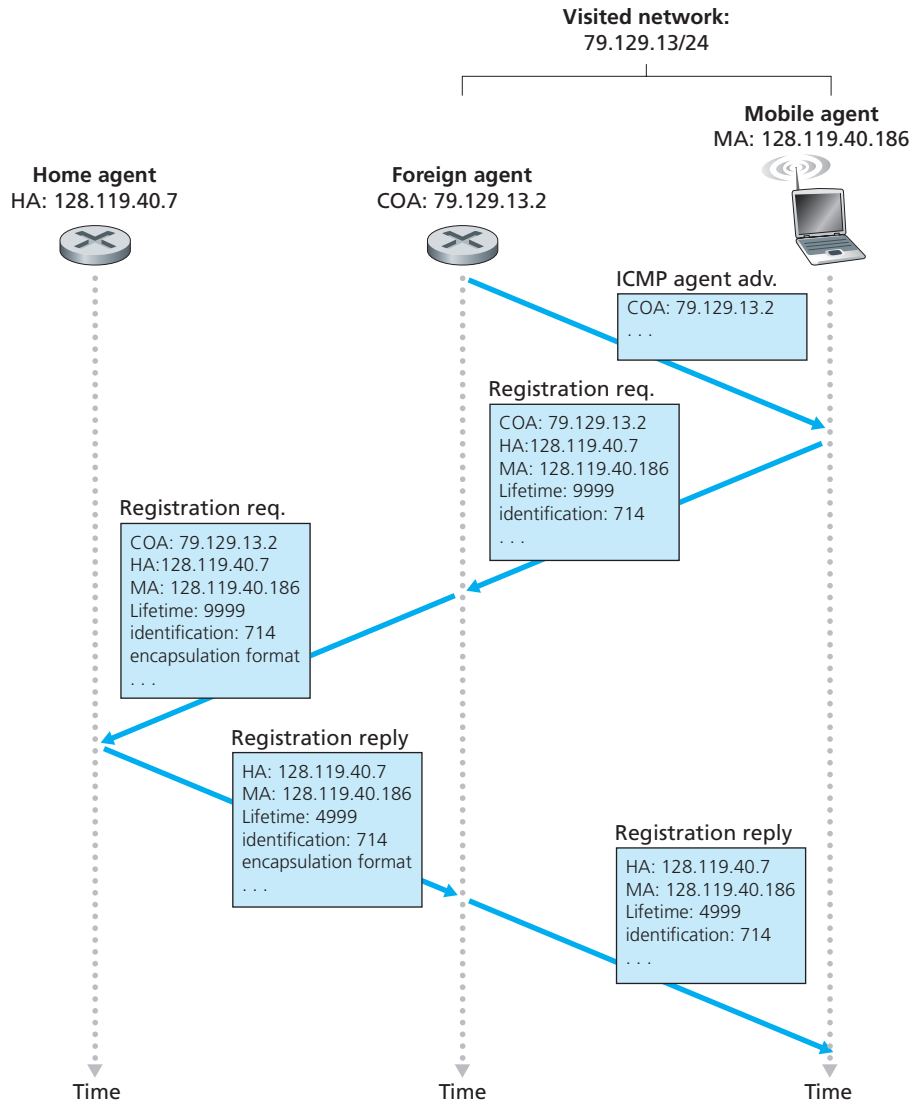
Figure 7.29 ♦ Agent advertisement and mobile IP registration
